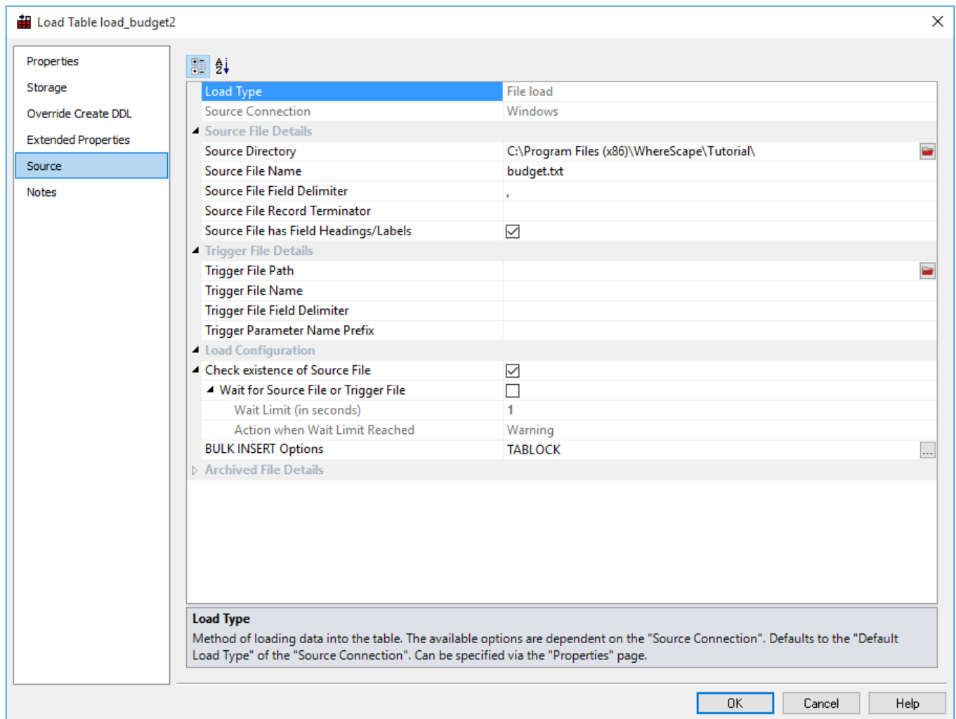
SQL Server Script load Source screen from a Windows connection:
